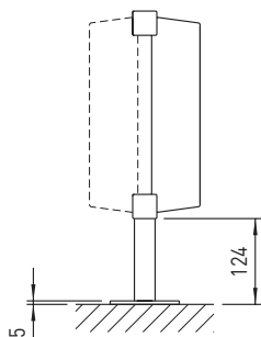
SF124 feet, Profilansicht
